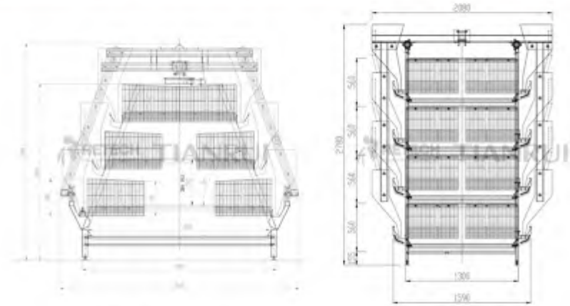
A Type Pullet Cage
