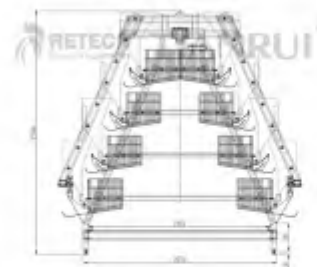
9TLD-4128 belt type
